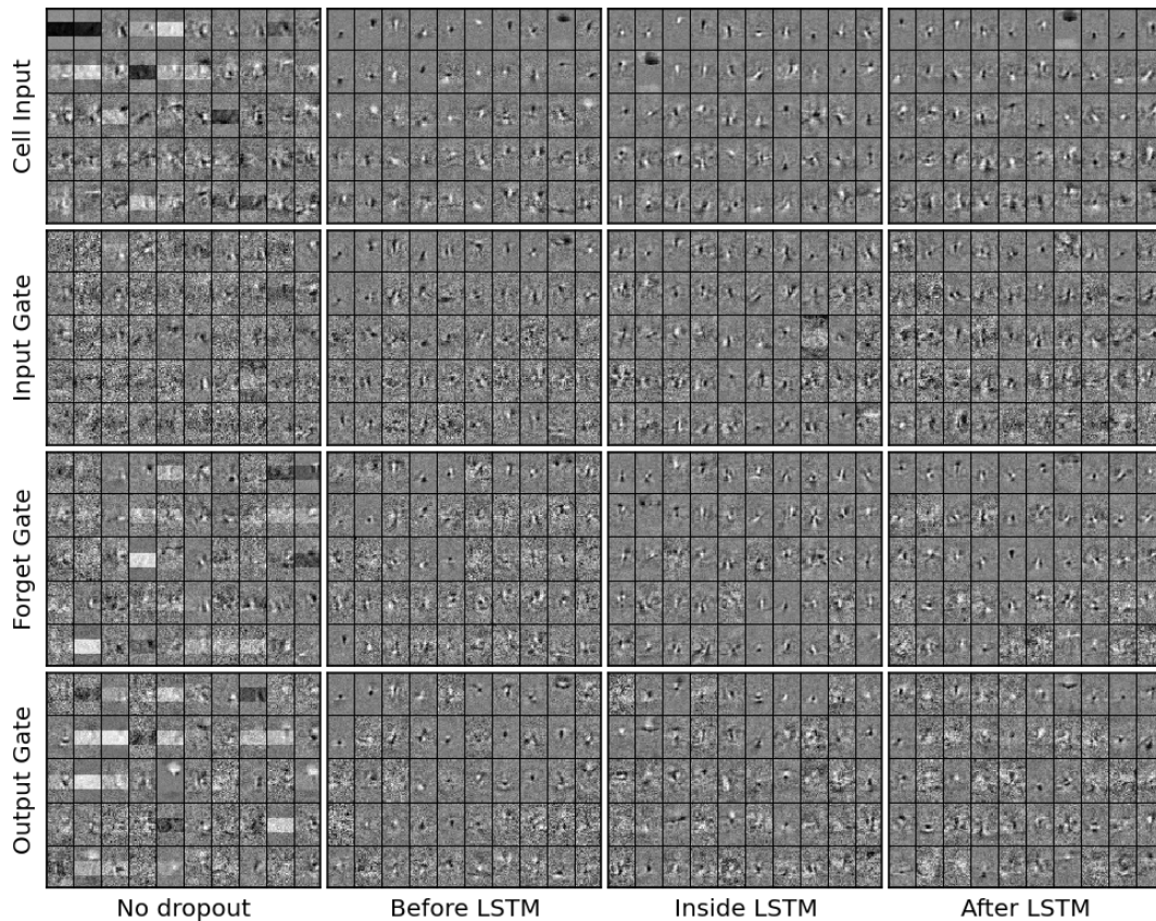
Figure 6.12: Weights of the first layer of pixel LSTM-RNNs with different dropout strategies on Rimes database ( Pix./Deep/CTC ).
